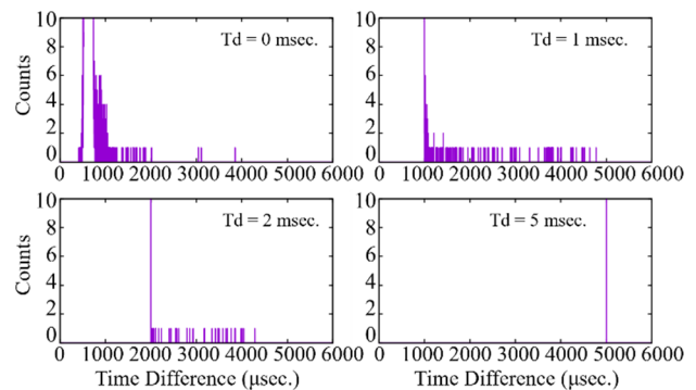
Figure 5: Time difference distributions for each T_d .
