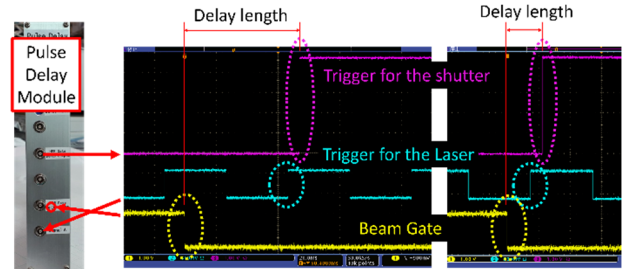
Figure 2: Waveforms of triggers for the shutter, triggers for the laser, and beam gate signals.
