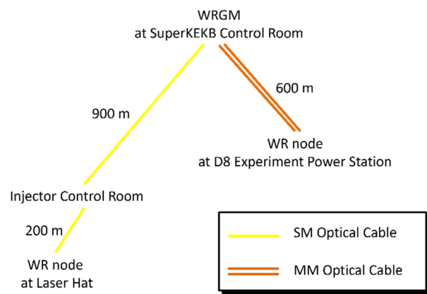
Figure 4: Diagram of the optical fiber path.
