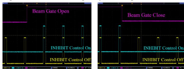
Figure 7: Picture of the beam gate system in operation.
